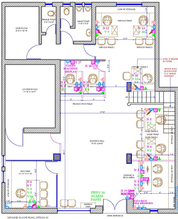
PROPOSED LAYOUT of "MATAR" BRANCH, KHEDA, STATE BANK OF INDIA
